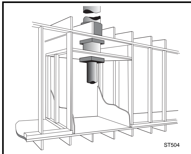
Fig. 24 Cutaway perspective of alcove installation.
