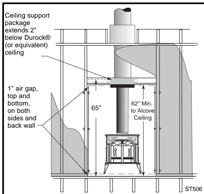
Fig. 26 Front view: 65" minimum clearance from hearth to combustibles on front face. Combustible facing may overlap metal studs by only 1". It should not extend below the height of the non-combustible ceiling.
