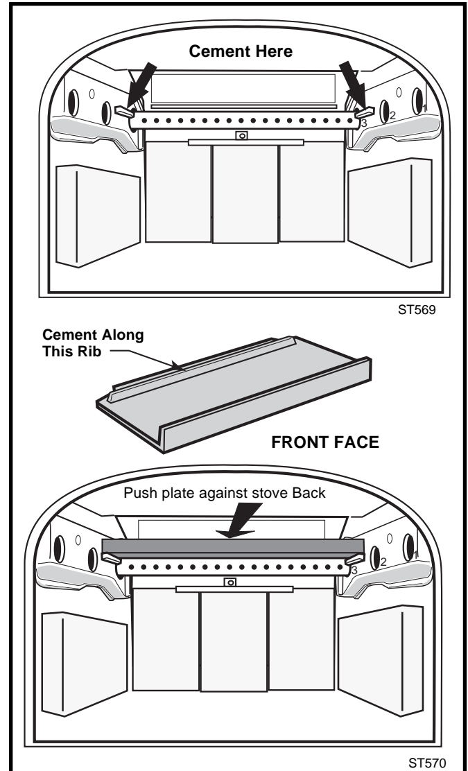
Fig. 29 Installing the Smokeshelf.
