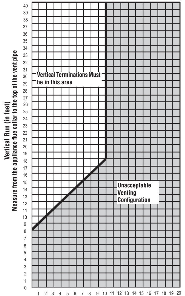
Figure 14 Horizontal Run (in feet)
